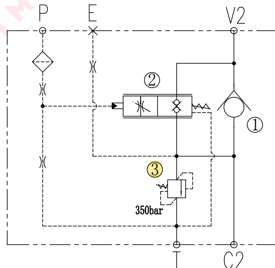
Hydraulic schematic
