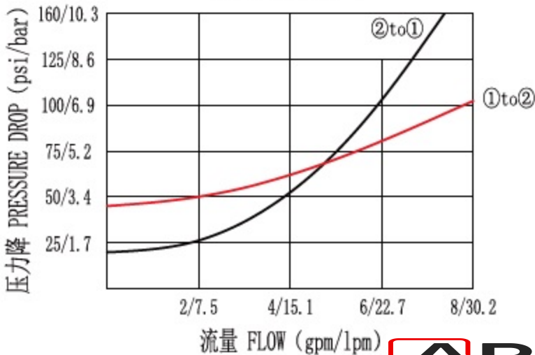
压力-流量曲线 PRESSURE DROP VS. FLOW
